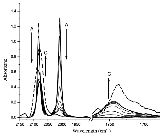
Fig. 1. Series of IR spectra {ν(CO) region} illustrating the reaction of 1b (A) with MeI at 25°C. The arrows indicate the behavior of each band as the reaction progresses. The bands of the products 2b (C) are broad and shouldered due to presence of a mixture of isomers. The dotted lines express the spectra after completion of the reaction.
