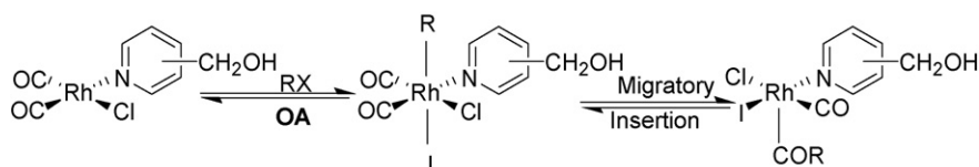
Scheme 2. OA reaction of RX with complexes 1 .
