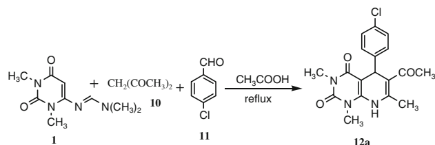
Scheme 5 Synthesis of pyridopyrimidine derivative 12a
