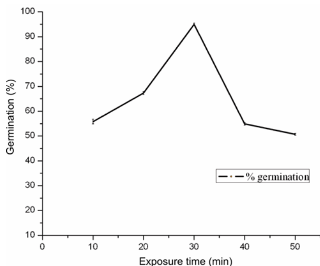
Figure 2. Germination percentage of encapsulated PLBs in relation to different exposure time to CaCl 2 ·2H 2 O solution. (After 10 weeks of culture.)
